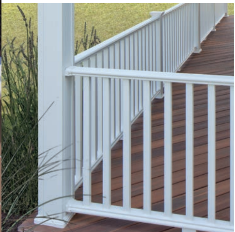
Kingston Railing with square balusters in white. Also shown is 6"x 6" Certa-Snap® Post Wrap.
