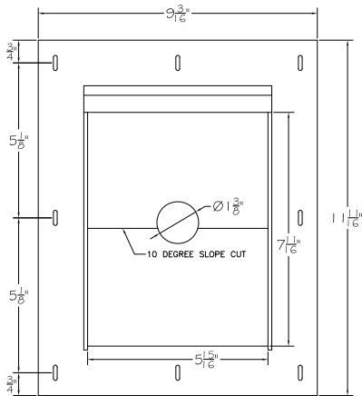
Split Block 6" x 8-1/2"
