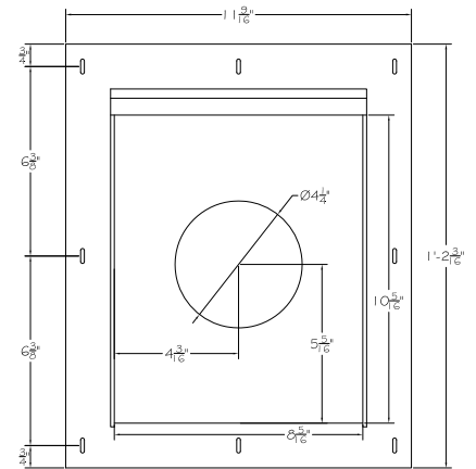
Universal 8-1/2" x 11"
