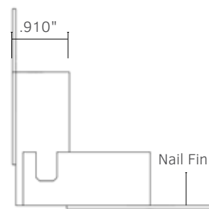
Inside Corner
