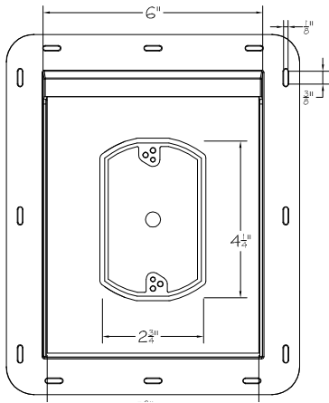
UL Electrical 5-3/4" x 7-3/4"
