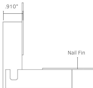
Outside Corner
