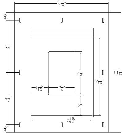
Receptacle 6" x 8-1/2"
